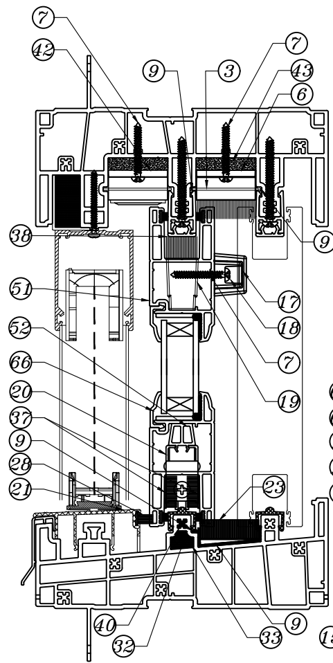
Section B-B
