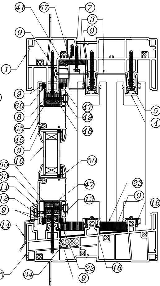
Section C-C
